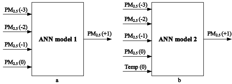
Fig. 3. ANN models
