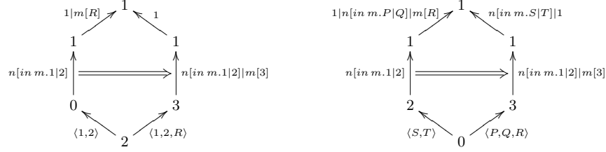
Fig. 5. G-luxes transitions originating from n[in\ m.1 | 2] .
