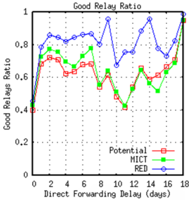
Fig. 4. Average Good Relay Ratio
