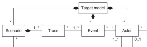
Fig. 4. Meta-model for generic target model
