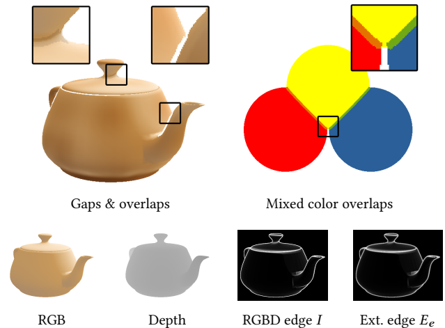
Figure 5: Results of gaps & overlaps in object-space and a breakdown of the edge extraction and edge extension.
