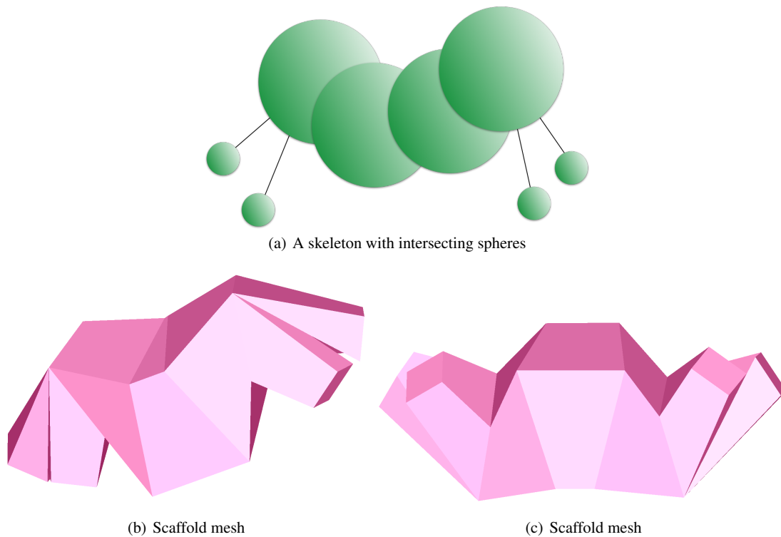
Fig. 8 The simple skeleton of Figure 7 with varying radii. The large radii lead to intersecting spheres at the interior vertices, but the faces remain quads.
