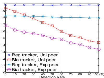
Fig. 8: Percentage of cross-AS traffic (a small torrent with 100 initial peers)
