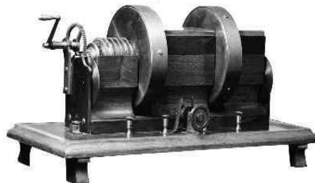
Figure 2.3: The Jedlik's Dynamo
