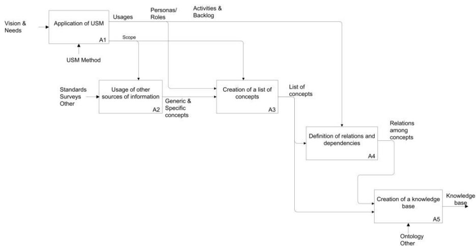
Fig. 2. Diagram displaying the creation of knowledge base
