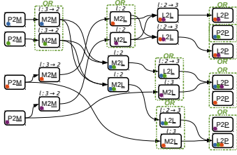
Fig. 6: Symbolic meta-DAG for the FMM associated with Figure 2b where tasks with an OR block can be executed in any order instantiated dynamically.
