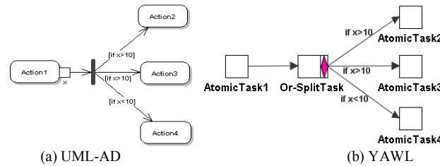
(a) UML-AD (b) YAWL Figure 11. Multi-Choice (Pattern 6) in UML-AD and YAWL
