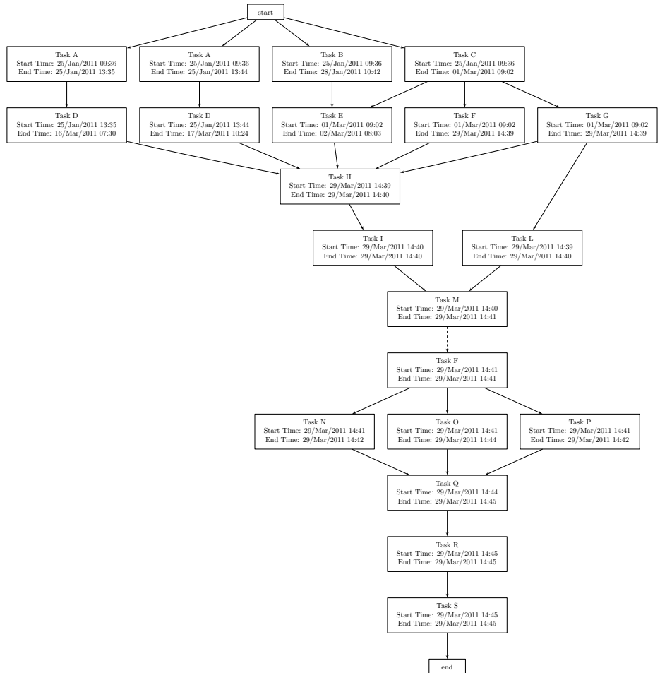
Fig. 7. Diagram showing pattern caused by staged executions
