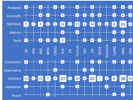
Figure 3: Modeling techniques by research type and contribution type.
