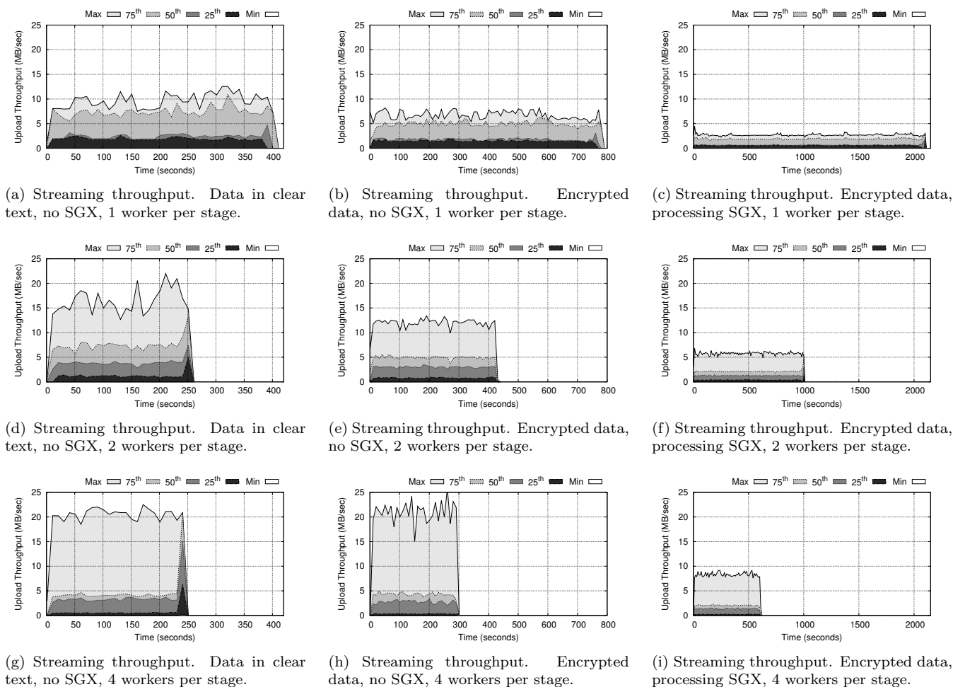
Figure 6: Throughput comparison between normal processing (with cleartext data and no encryption), encrypted data but without enclaves, and with encrypted data and SGX processing. We scale the number of worker nodes per stage from 1 (left-most column), 2 (center column) and 4 (right-most column).
