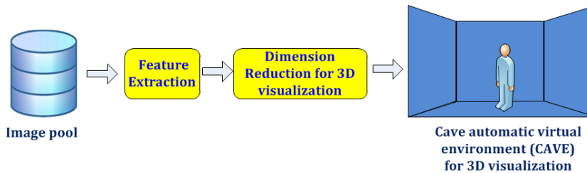
Fig. 2. An immersive visualization system provides the user with a visual representation of data. Here, high-dimensional features are extracted from a database of Earth Observation images and are fed into a dimension reduction technique to be visualized in an immersive 3D virtual environment.
