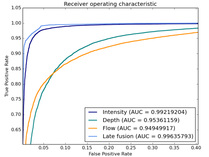
(b) Incremental cross-modality
