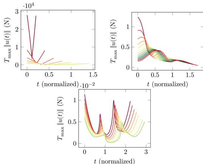
Figure 15: Controls for different transfer times for the transfer between invariant manifolds from Halo orbits in the {Earth-Moon} system. Left: small times, similar to \Delta V . Center: Longer times. Right: After the interval I_{SE} , where the algorithm fails, a different structure for the control is obtained corresponding to a trajectory with a revolution. The different colors are for the steps of the continuations.
