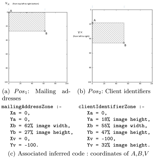
Fig. 7. Automatic inference of position operators for senderDetails elements. Two groups of positions are automatically detected, Pos_1 and Pos_2 . The semantic name of the positions is provided by the user.
