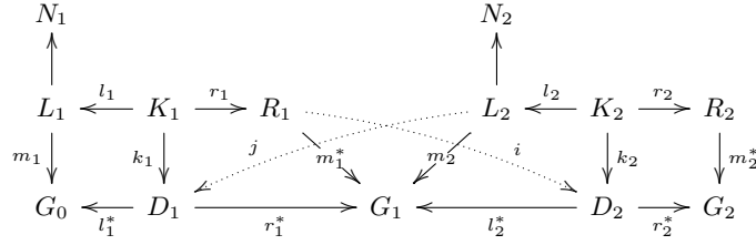
Fig. 2. Sequential independence
