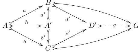
Fig. 7. Quasi-pushout of monos in an adhesive category
