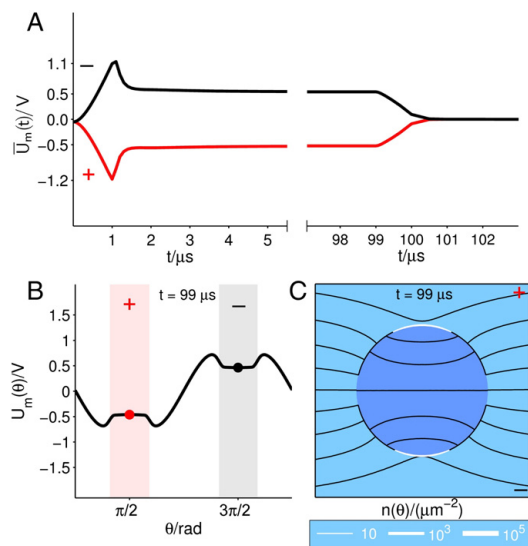
Figure 5. Numerical simulations of KN-model from Figure 3 of [28] (Courtesy of J.C. Weaver). ”Electrical and poration response to a 1 kV/cm, 100 \mu\text{s} trapezoidal pulse with 1 \mu\text{s} rise and fall times. (A) Transmembrane voltage spatially averaged over the polar quadrants, during the initial 5.5 \mu\text{s} , and at the end of the pulse from 97 to 103 \mu\text{s} . Red ‘+’ indicates the hyperpolarizing anodic side and black ‘-’ indicates the depolarizing cathodic side. (B) Angular profile of transmembrane voltage at 99 \mu\text{s} . Background shaded regions indicate the angular extent of EP around the anodic and cathodic sides of the membrane. Red and black dots mark the location of the anodic and cathodic poles on the membrane, respectively. (C) Equipotentials (black) and pore density, n(\theta) (white), at 99 \mu\text{s} .”
