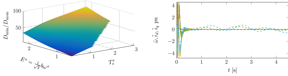
(a) Minimum required damping coefficient D_{\min} compared to nominal damping coefficient D_{\text{nom}} for condition (3.16) to be satisfied in a broad range of operating conditions. (b) Simulation results for the system (3.5). The solid lines show the state trajectories of \tilde{\omega}, \tilde{i}_d, \tilde{i}_q for the case d(t) = \underline{0}_3 . The dashed lines correspond to the case d_1 = 0.25 \sin(3t) , d_2 = 0.5 \sin(5t) , d_3 = 0.3 \sin(t) .
