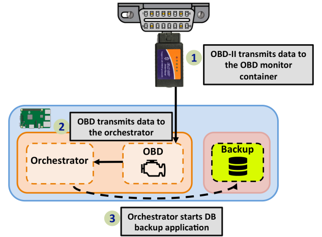
Fig. 3. Data Base Container activation.
