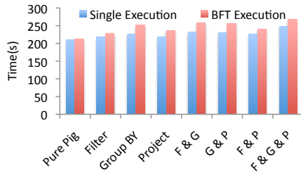
Fig. 9: Latency of running Twitter Follower Analysis
