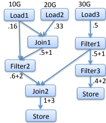
Fig. 4: Annotated data-flow graph
