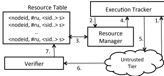
Fig. 6: Execution tracker & resource manager
