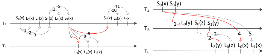
Fig. 2: Pruning constraints implied by previous constraints. Fig. 3: Example of partial transitive reduction.
