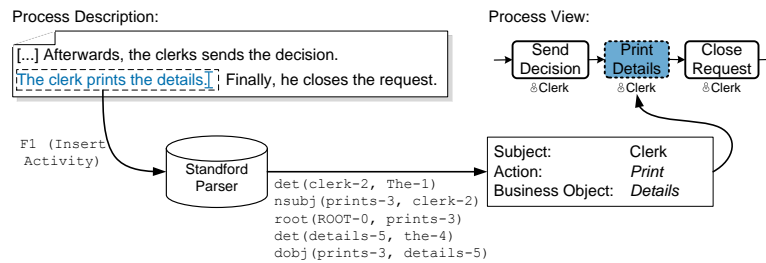
Fig. 6. Inserting a Sentence and Adapting the Corresponding Process View
