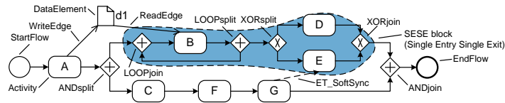
Fig. 2. Example of a Process Model
