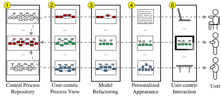
Fig. 3. Overview of proView Framework
