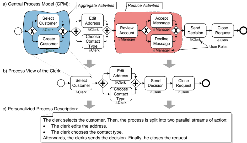
Fig. 5. Creating a Personalized and Verbalized Process Description
