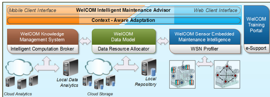
Fig. 1. WelCOM e-Maintenance Architecture
