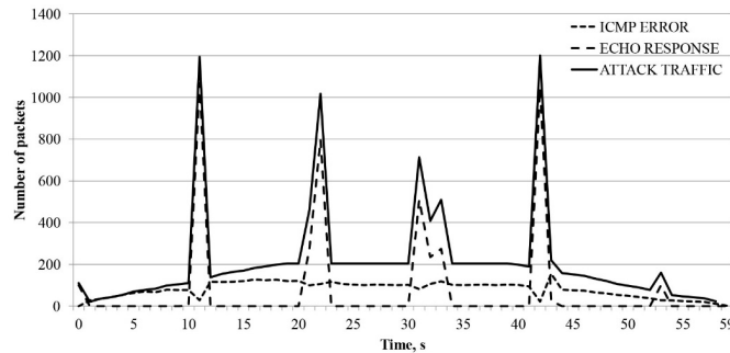
Fig. 8. Server traffic under an Echo attack with bounced traffic
