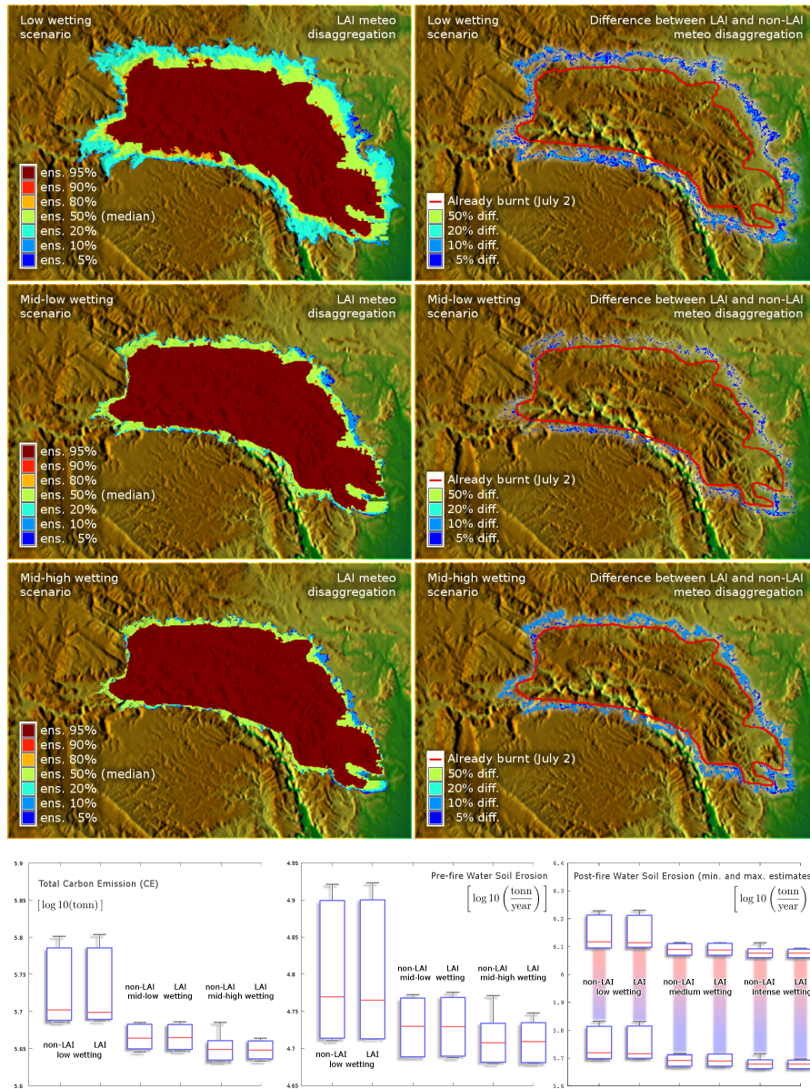
Fig. 2. Dos Aguas, Valencia – Spain. Wildfire behaviour simulations with ensemble prediction (July 3 2012). To illustrate, simplistic fire control scenarios are shown: low wetting ( top ); mid-low wetting ( middle ) and mid-high wetting ( bottom ). Interpolation driven uncertainty (IDU) is also assessed. Meteorological forecasts have been spatially disaggregated by either imposing local average invariance (LAI) [24] ( left ) or not (usual non-LAI disaggregation). The difference is shown at right . Below: rapid assessment of wildfire impacts. Total carbon emission and soil erosion by water (pre- and post-fire) have been estimated for each ensemble simulation of each scenario. Box-plots: box with quartiles 25%, 50% (red line), 75%; whiskers with 5% and 95% quantiles. Although the assessment considers the whole burnt area and not only the one which would have been burnt in the simulated day under the different scenarios, the non-LAI induced component of IDU is nonlinear and even its one-day effects may occasionally be non-negligible for the impact assessment of the whole burnt area.
