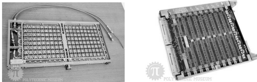
Fig. 13: The processor block and the operative memory block of the “Electronica SS BIS-1” super computer
