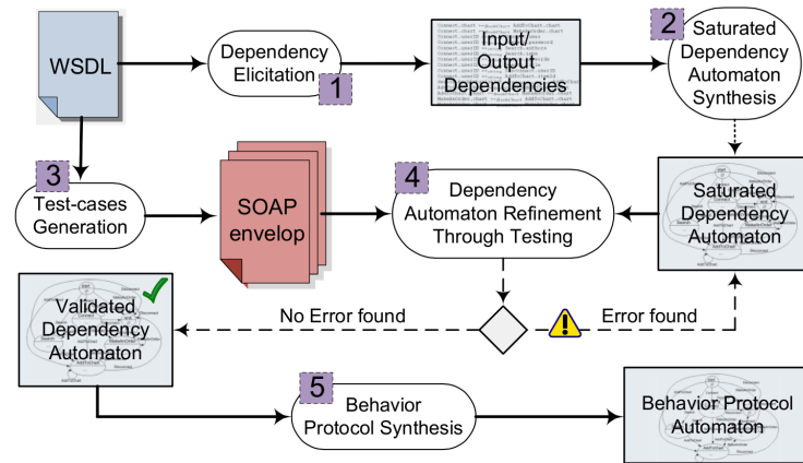
Fig. 2. Overview of the StrawBerry technique
