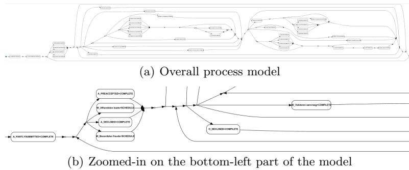
Fig. 10. Algorithm: Inductive miner [22]. Result in ProM for the BPIC 2012 event log.
