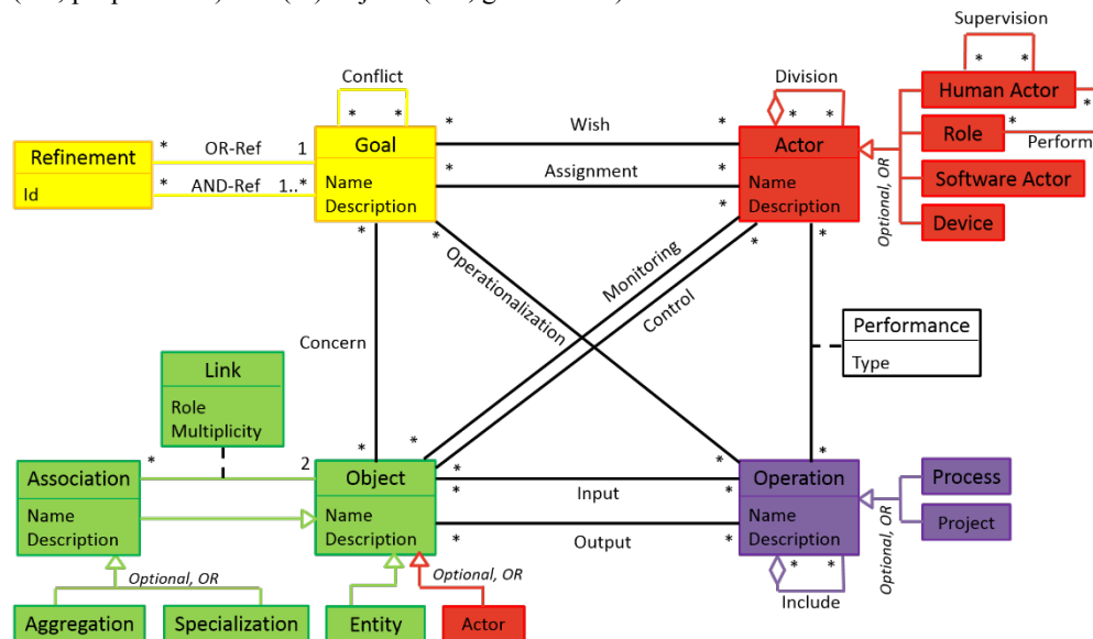
Fig 1. CHOOSE metamodel [8]
