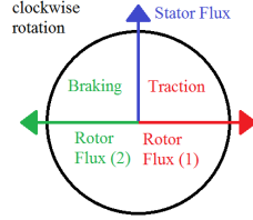
Fig. 3. Fluxes positioning and effect
