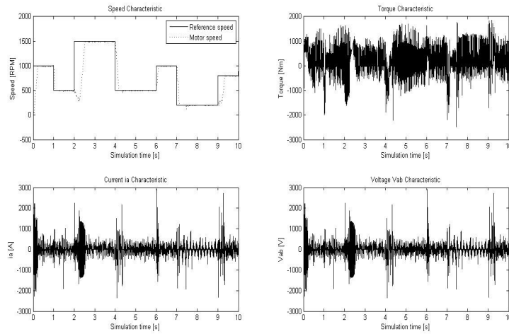
Fig. 6. Results for 100 Nm load.
