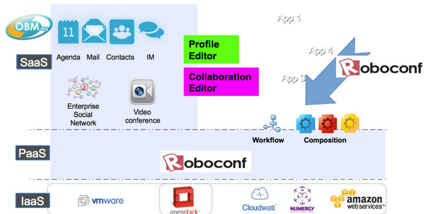
Fig. 1. OpenPaaS Platform.
