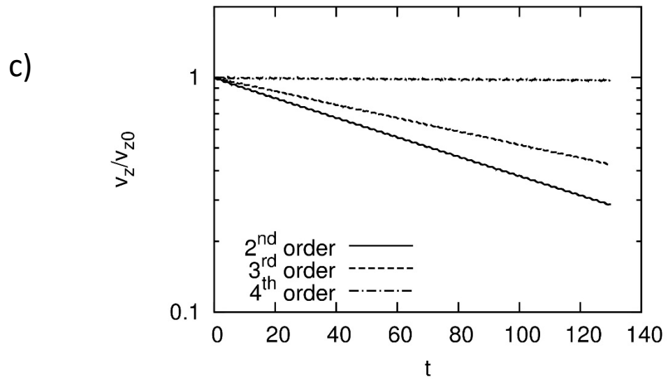
Figs. 9a and 9b show the evolution of the maximum z-velocity and maximum z-component of the magnetic field in the relativistic torsional Alfvén wave as a function of time. For the simulations shown in Figs. 9a and 9b we used the 1D HLLI Riemann solver along with the 2D MuSIC Riemann solver with sub-structure. Figs. 9c and 9d show the same information as Figs. 9a and 9b, the only difference being that we used the 1D HLL Riemann solver along with the 2D MuSIC Riemann solver without sub-structure.
