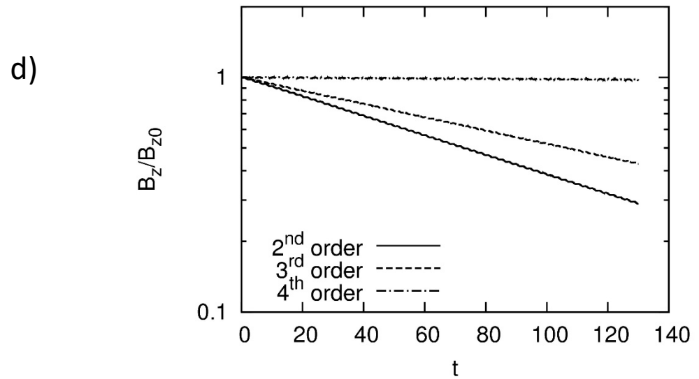
Figs. 9a and 9b show the evolution of the maximum z-velocity and maximum z-component of the magnetic field in the relativistic torsional Alfvén wave as a function of time. For the simulations shown in Figs. 9a and 9b we used the 1D HLLI Riemann solver along with the 2D MuSIC Riemann solver with sub-structure. Figs. 9c and 9d show the same information as Figs. 9a and 9b, the only difference being that we used the 1D HLL Riemann solver along with the 2D MuSIC Riemann solver without sub-structure.
