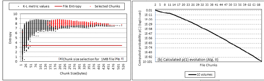
Fig. 2. Chunk optimal size computation[3]
