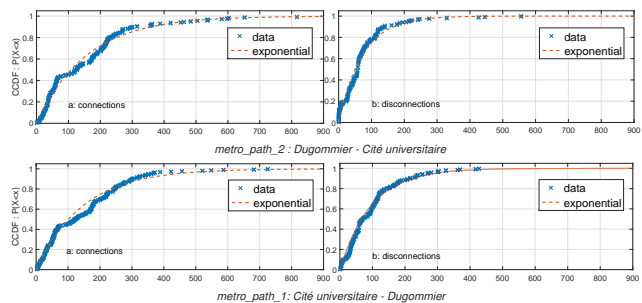
Figure 10: CCDF of connections and disconnections.
