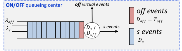
Figure 5: ON/OFF queueing center.
