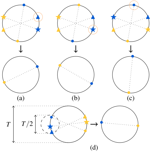
Fig. 4 Estimating the average of poses with multiple representatives: illustration with the orientation of a 2D object with a 180° rotation symmetry, that can be represented by a point on a circle, or the antipodal point. We consider three poses to average (triangle, star and disk shapes). (a, b, c) The choice of a “consistent” combination of poses representatives (blue clusters) in the sense of (Gramkow 2001) is dependent of the initial choice (circled, first row), resulting potentially in different estimations of the average pose (second row). (d) We propose a definition of consistency – which is in particular satisfied when the considered representatives are close enough one an other – ensuring an unambiguous estimation of the average pose.
