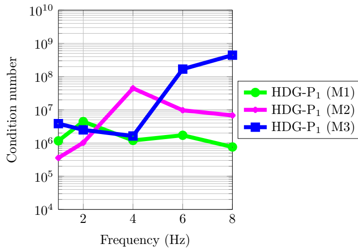
Figure 5.13: Condition number of the HDG- P_1 matrix as a function of the frequency.
