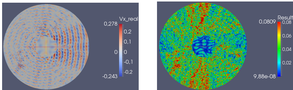
(a) Numerical solution, mesh M2, HDG- \mathbb{P}_2 scheme, V_x component.
