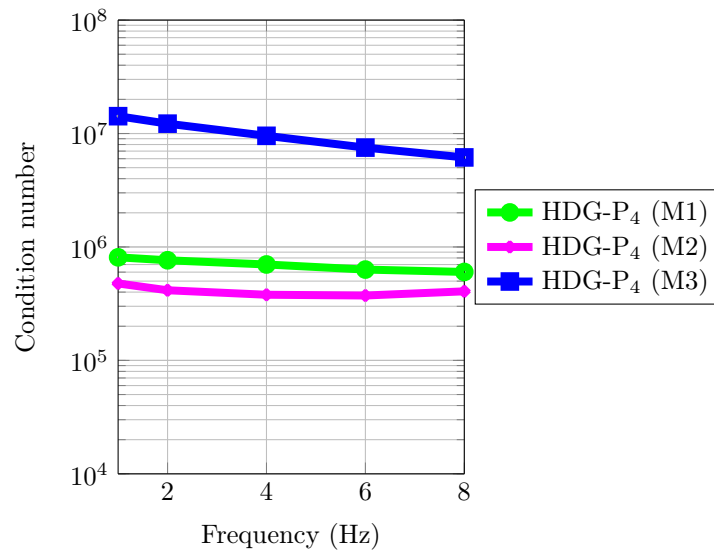
Figure 5.16: Condition number of the HDG- P_4 matrix as a function of the frequency.
