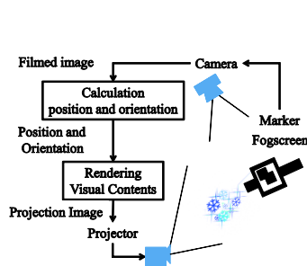
Fig. 1. System Flow
