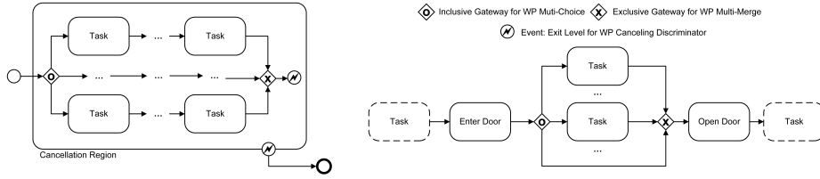
Fig. 3. Left: General FPS workflow pattern for HL2. Right: Exploded BPMN view of tasks in the left image, illustrating how the door opening tasks are key to enforcing particular orderings of tasks in HL2 as an FPS.
