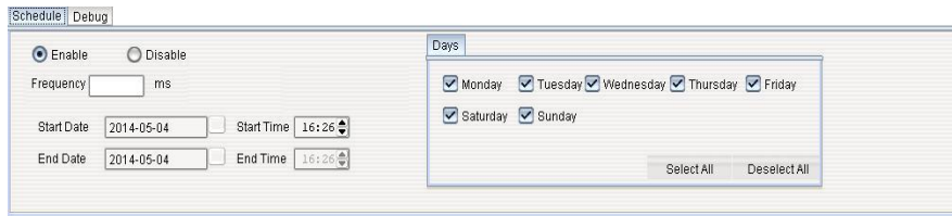
Fig. 4. Script Scheduler
