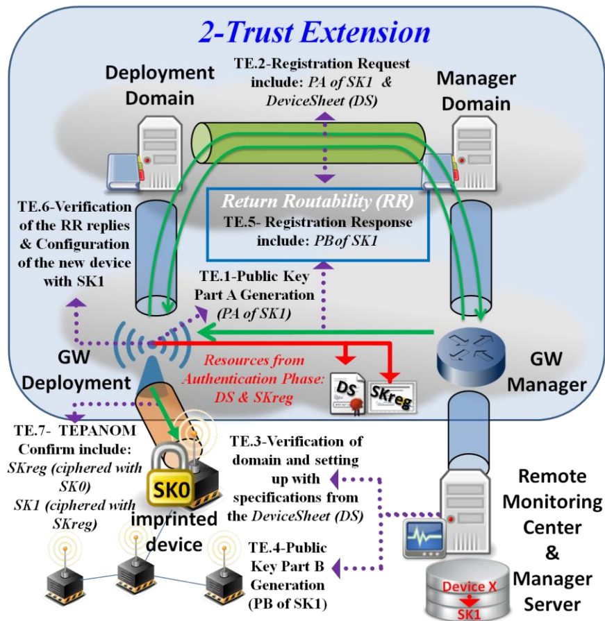
Fig. 3. TEPANOM Trust Extension Phase.
