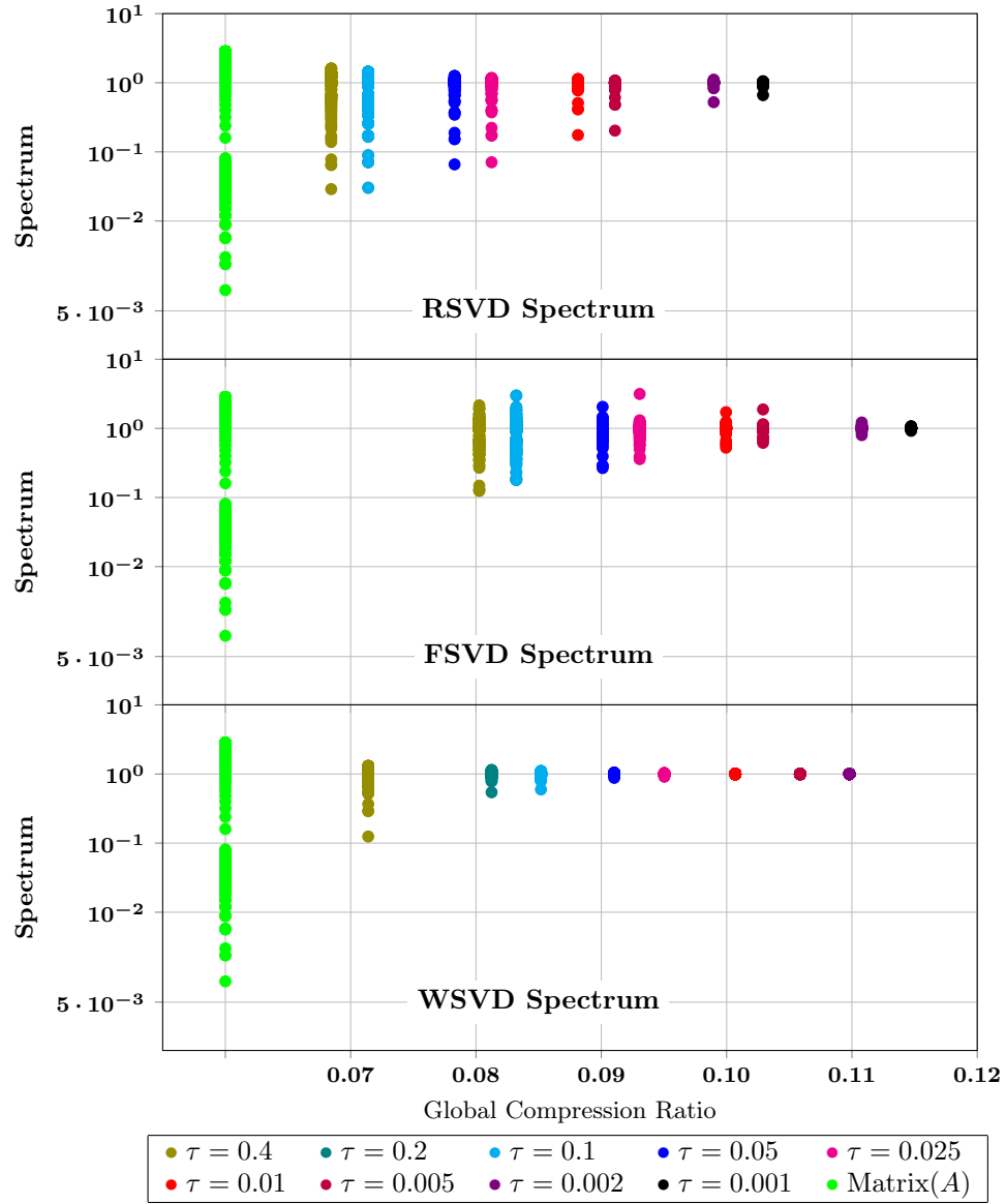
Figure 7: Spectrum Clustering of the Preconditioned system.
