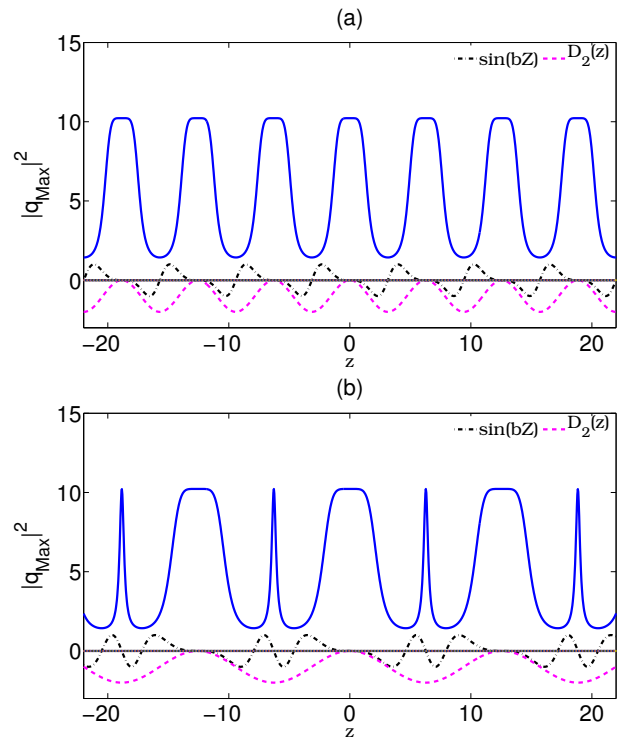
FIG. 3. (Color online) The shape of the generalized Kuznetsov-Ma soliton with periodic coefficients as a function of z with d_m = 1 and a = 0.603 . (a) k_m = b , (b) k_m = b/2 .
