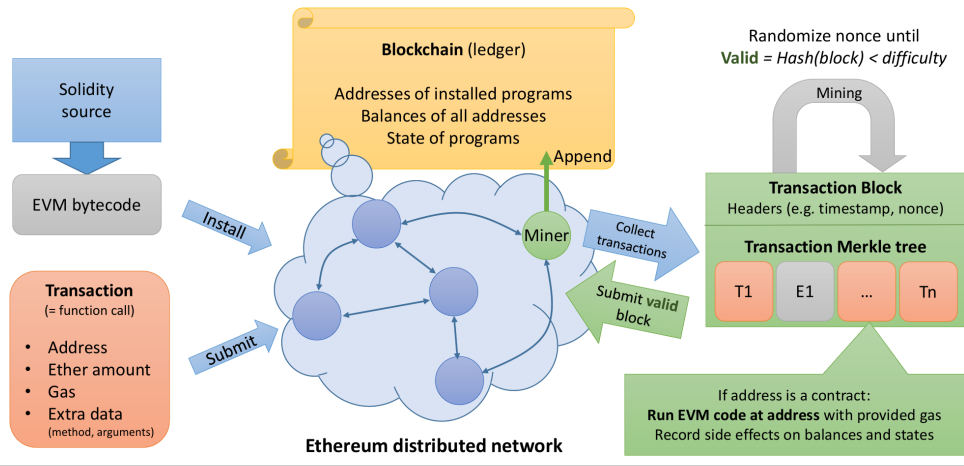
Figure 1: Overview of workflow in the Ethereum network
