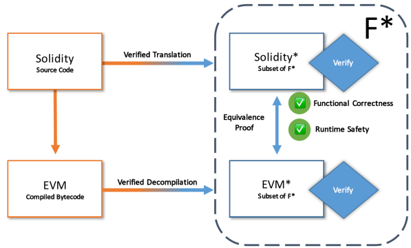
Figure 2: Outline of our verification architecture
