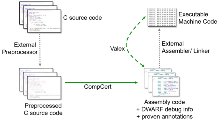
Fig. 1. CompCert Workflow
