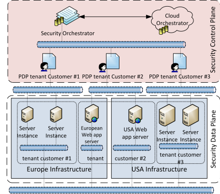
Figure 2. Use-case for supporting the validation of our SDSec architecture
