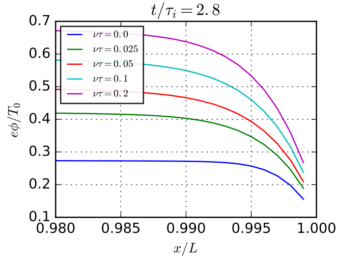
Figure 12. Electric potential profile near the wall at t \approx 2.8\tau_i for a time-distributed source.
