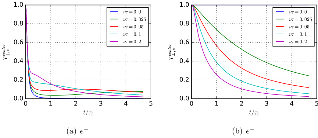
Figure 3. Electron parallel (a) and perpendicular (b) temperatures at x = 0 .
