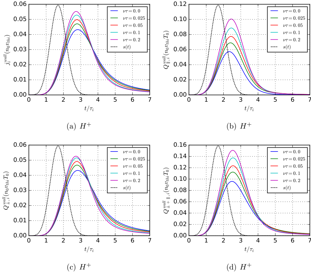
Figure 10. Ion fluxes at the target plate for a time-distributed source: (a) Particle flux; (b) parallel energy flux; (c) perpendicular energy flux; (d) total energy flux.
