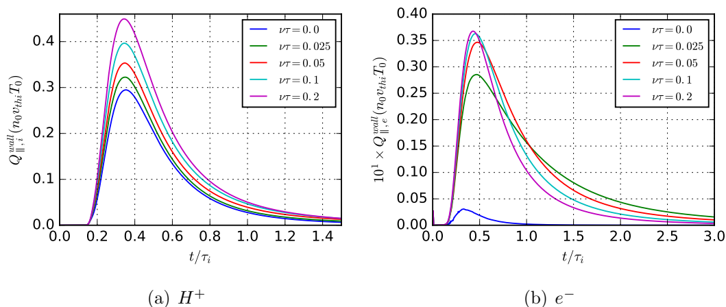
Figure 5. Temporal evolution of the ion (a) and electron (b) parallel energy fluxes at the right wall x = L .
