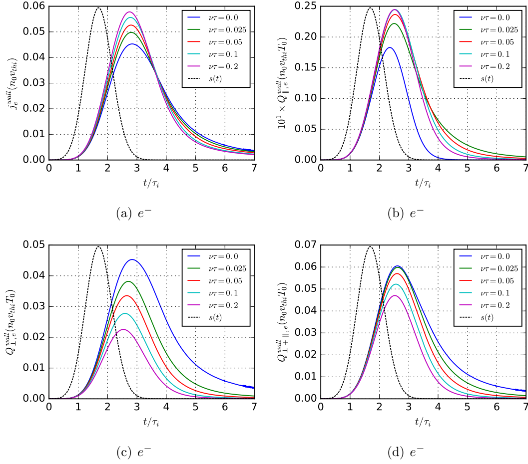
Figure 11. Electron fluxes at the target plate for a time-distributed source: (a) Particle flux; (b) parallel energy flux; (c) perpendicular energy flux; (d) total energy flux.
