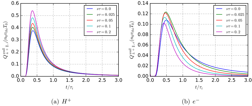
Figure 8. Ion (a) and electron (b) total energy fluxes Q_{\perp+\parallel}^{wall} at the right plate x = L .
