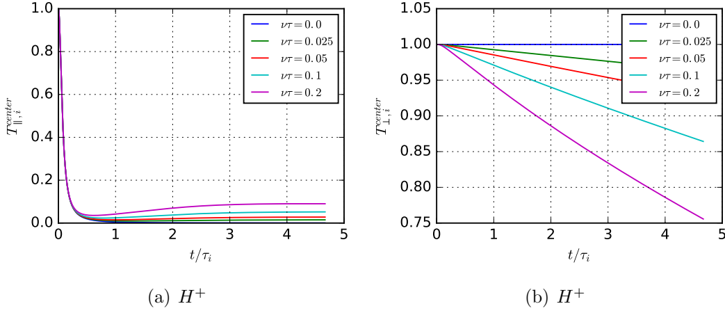
Figure 2. Ion parallel (a) and perpendicular (b) temperatures at x = 0 , for different collisionalities.
