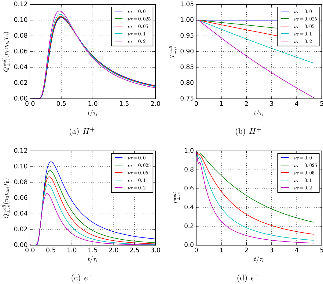
Figure 7. Temporal evolution of the perpendicular energy fluxes (left frames) and perpendicular temperatures (right frames) at the right plate x = L , for ions (top) and electrons (bottom).
