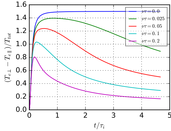
Figure 4. Electron temperature anisotropy T_{\perp,e} - T_{\parallel,e} normalized to the total temperature.
