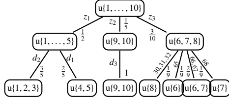
Fig. 5: The attack tree for Ex. 4. Leaves with the same label and their incoming arcs have been coalesced.
